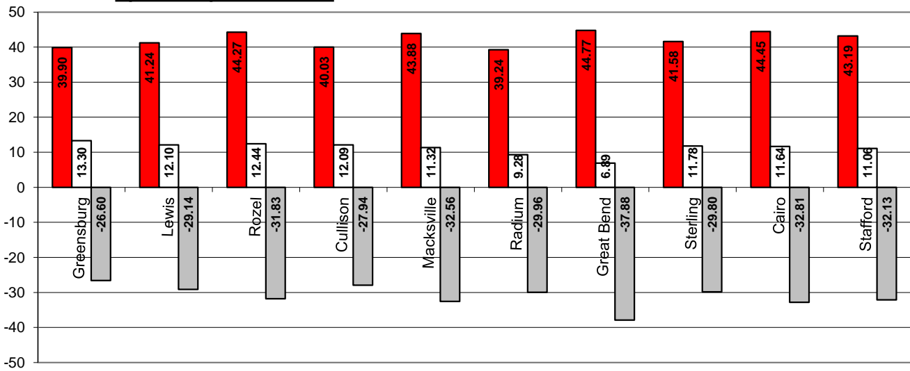
Big Bend GMD 5 Station Network Growing Season ET vs Rain Graph April to September, 2012
