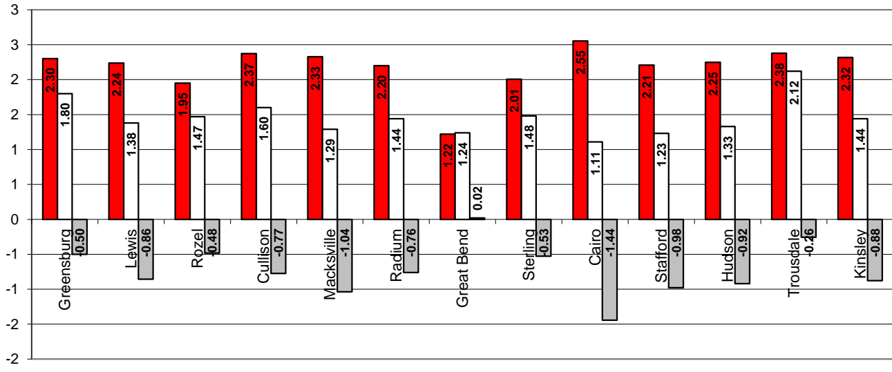
** Big Bend GMD 5 Station Network 2024 Yearly Graph ET vs Rain
