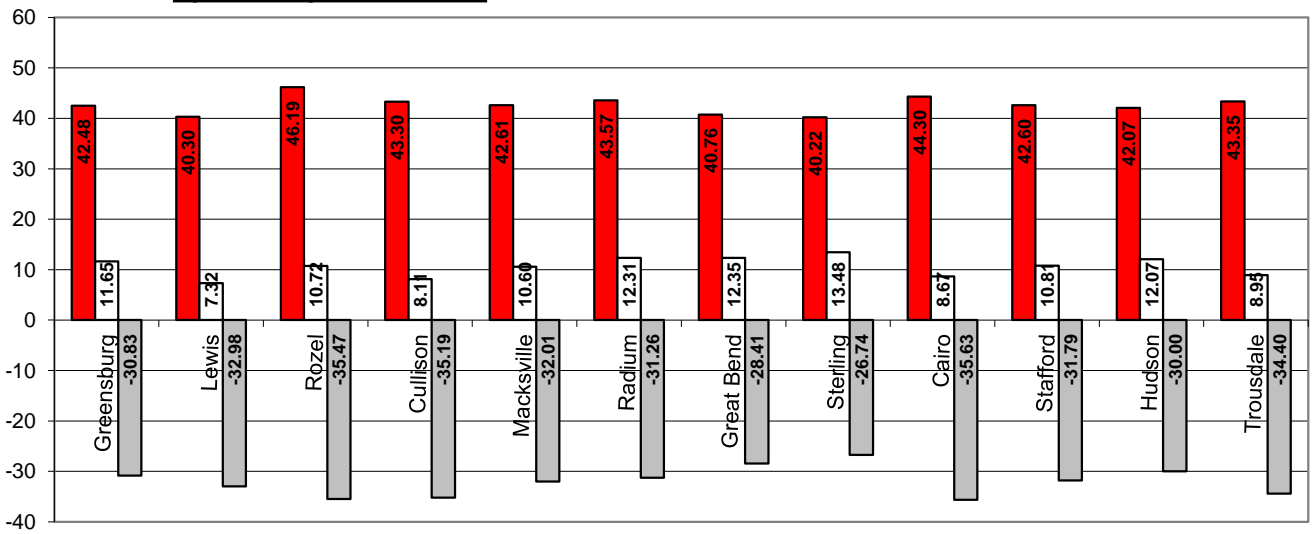
** Big Bend GMD 5 Station Network Growing Season ET vs Rain Graph April to September, 2022
